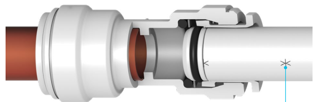
Pipe mark not level with collet head – indicating pipe not pushed fully home
